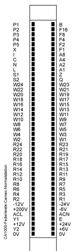
Normalstation 1-24
