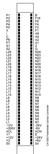
Controllerstation 0
